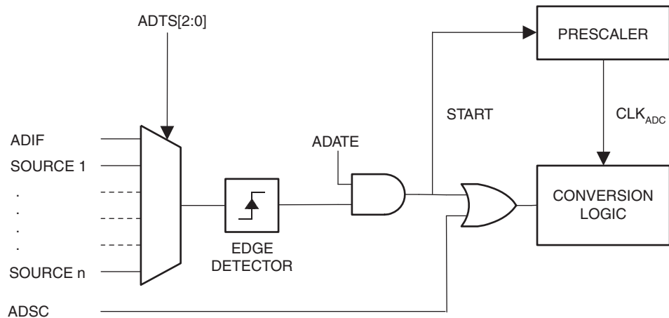
Figure 26-2. ADC Auto Trigger Logic
