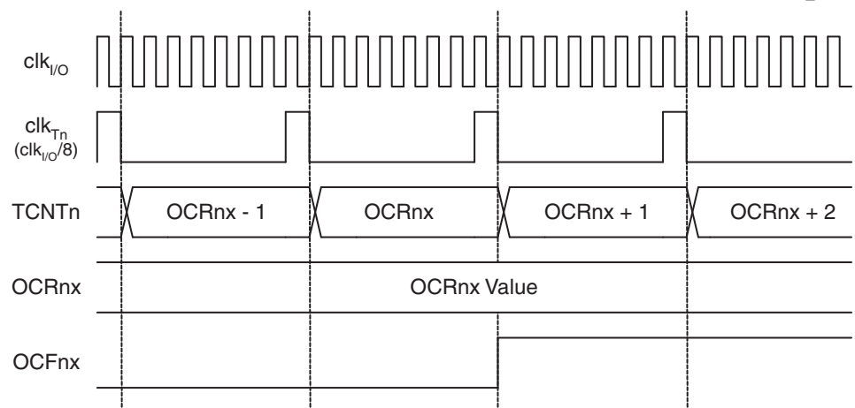
Figure 17-11. Timer/Counter Timing Diagram, Setting of OCFnx, with Prescaler ( f_{\text{clk}_{I/O}}/8 )
