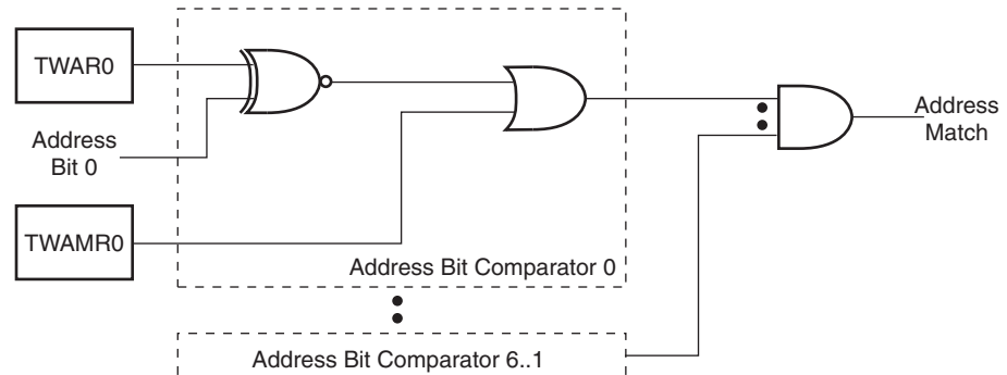
Figure 24-22. TWI Address Match Logic, Block Diagram
