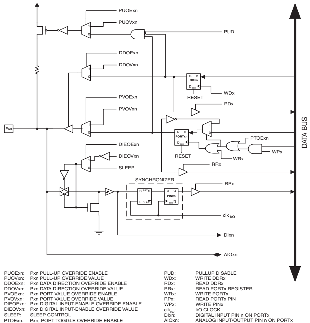
Figure 13-5. Alternate Port Functions (1)
