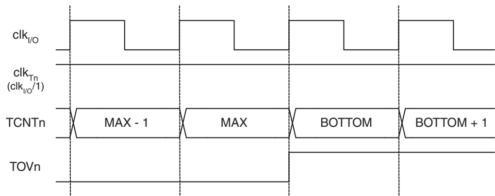
Figure 20-8. Timer/Counter Timing Diagram, no Prescaling
