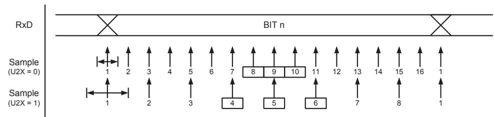
Figure 22-6. Sampling of Data and Parity Bit
