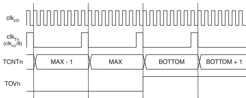
Figure 20-9. Timer/Counter Timing Diagram, with Prescaler ( f_{\text{clk}_{I/O}}/8 )
