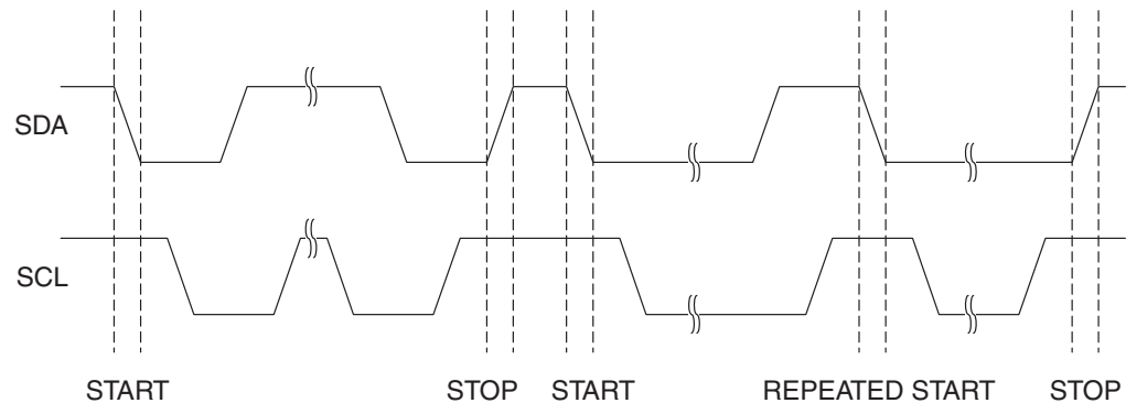
Figure 24-3. START, REPEATED START and STOP conditions
