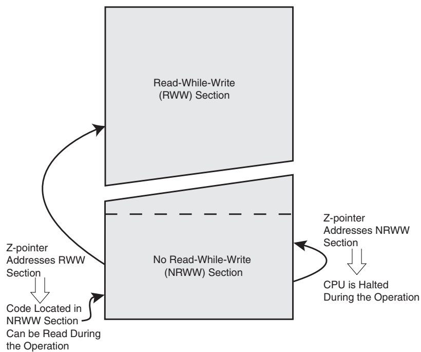
Figure 29-1. Read-While-Write vs. No Read-While-Write
