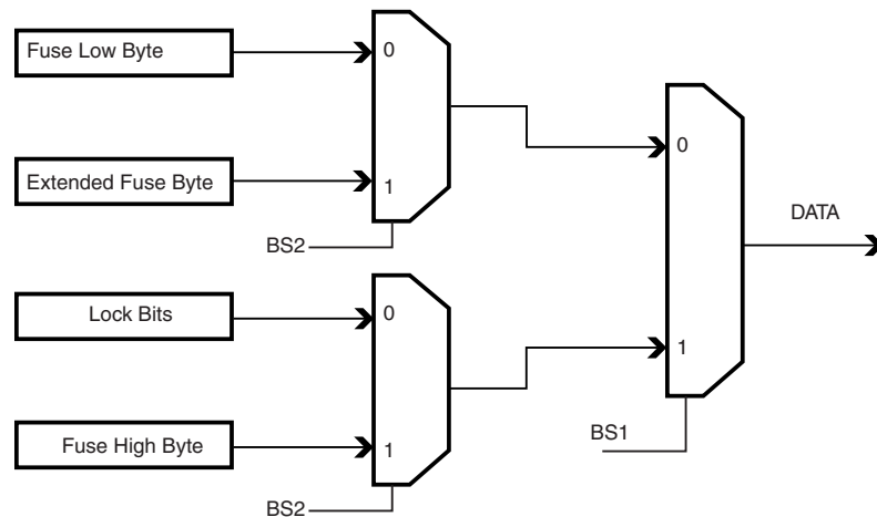
Figure 30-6. Mapping Between BS1, BS2 and the Fuse and Lock Bits During Read
