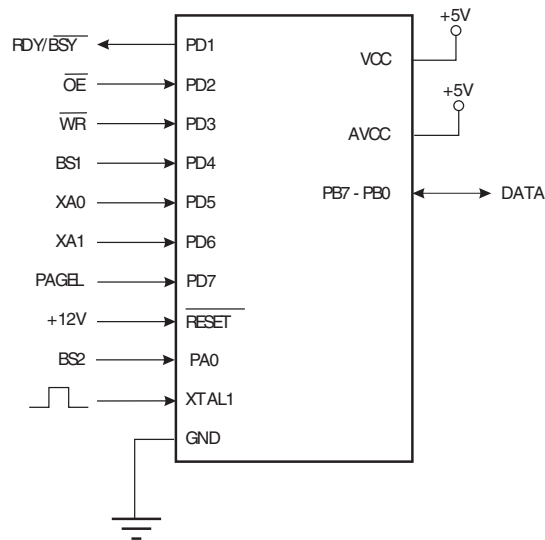
Figure 30-1. Parallel Programming (1)
