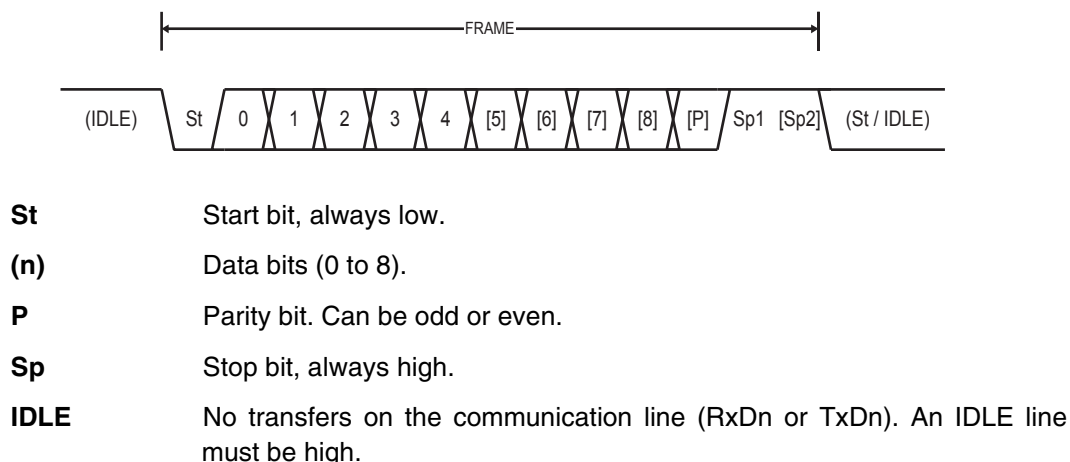
Figure 22-4. Frame Formats
