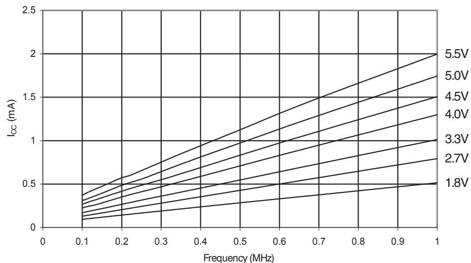
Figure 32-1. Active Supply Current vs. frequency (0.1MHz - 1.0MHz)
