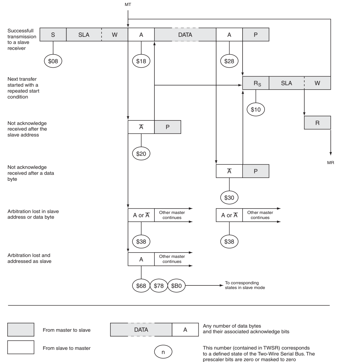
Figure 24-12. Formats and States in the Master Transmitter Mode
